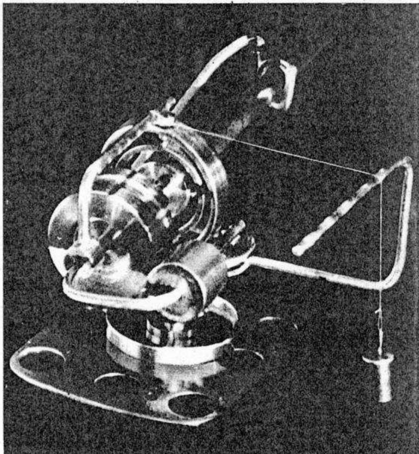
Rear view of mounting post and weighting arrangements for author's pickup arm.
