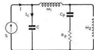
C_p and R_p are the Compliance and Resistance, respectively, of the coupling
