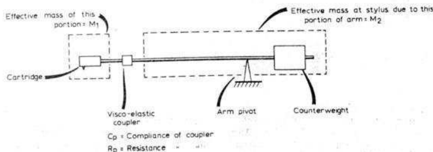
Fig. 9. Physical arrangement of dynamic damping parameters.
